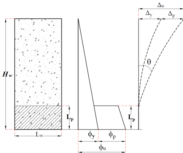
Figure 1. Theoretical model of elastic and plastic displacements in cantilever RC shear wall
