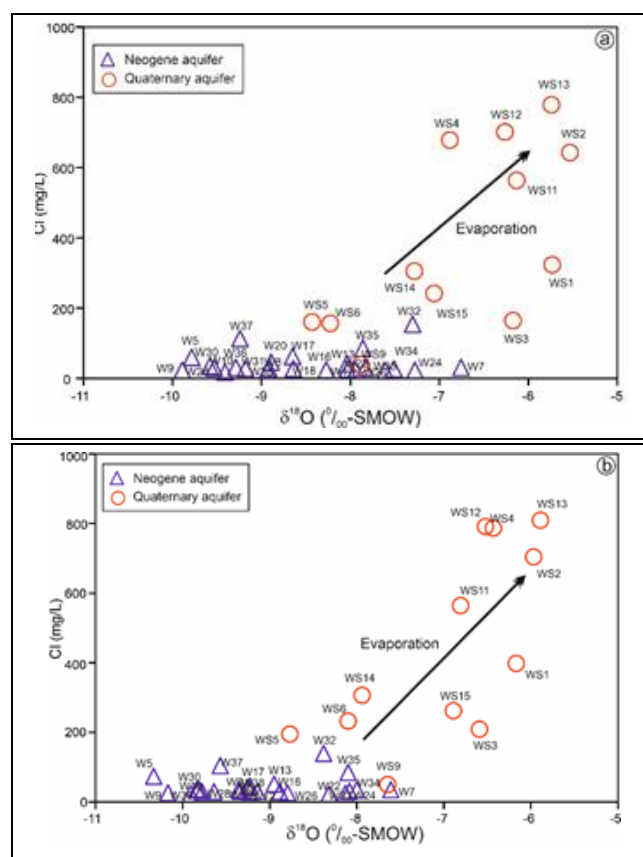
Figure 5. Relationship of \delta^{18}\text{O} and Cl (mg/L) in groundwater of both Neogene and Quaternary aquifers for, (a): Dry season, (b): Wet season.
