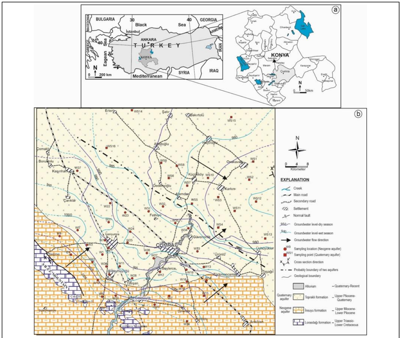
Figure 1(a): The location map and (b): Geological (modified from [11]-[14]), hydrogeological maps and groundwater sampling locations.
