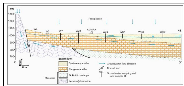
Figure 2. Conceptual hydrogeological cross section (X-X') of the Figure 1(b) (modified from [9]).
