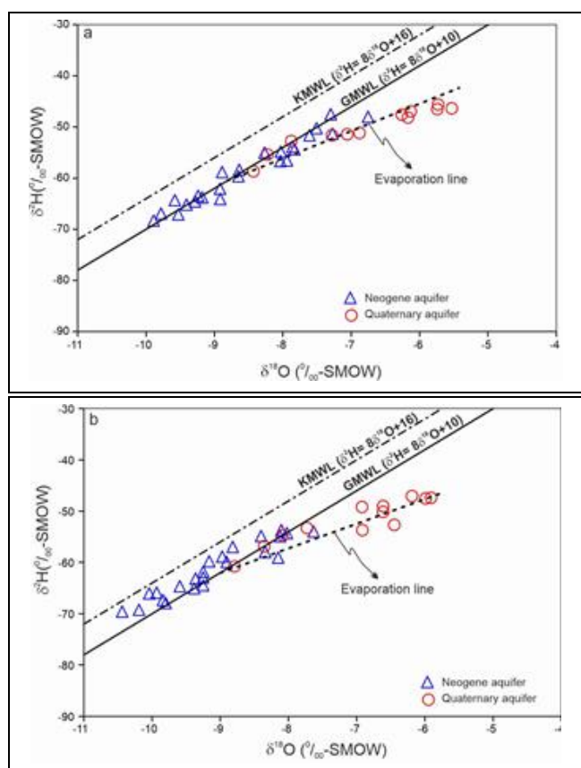
Figure 4. Relationship of \delta^2\text{H} and \delta^{18}\text{O} in groundwater of both Neogene and Quaternary aquifers for, (a): Dry season and (b): Wet season.
