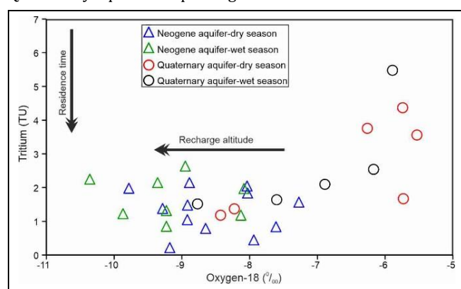
Figure 8. The relationship between \delta^{18}\text{O} (‰) and tritium (TU) in groundwater of both Neogene and Quaternary aquifers.
