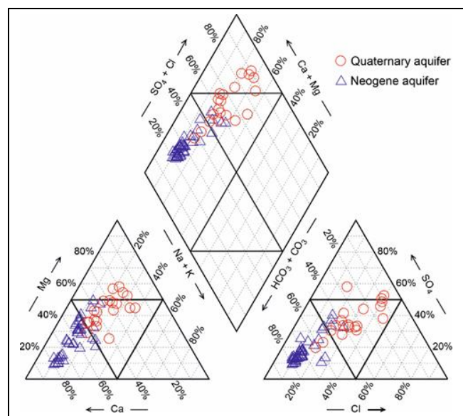
Figure 3. Piper diagram of the Neogene and Quaternary aquifer samples (taken from [9]).
