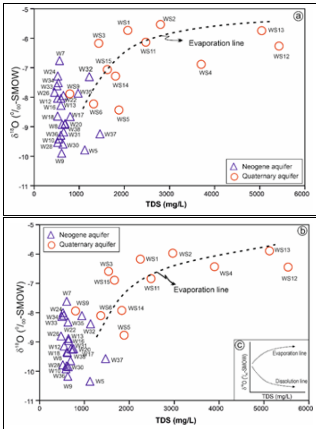
Figure 6. Relationship of \delta^{18}\text{O} and TDS (mg/L) in groundwater of both Neogene and Quaternary aquifers for, (a): Dry season, (b): Wet season, (c): \delta^{18}\text{O} - TDS relationship [21].
